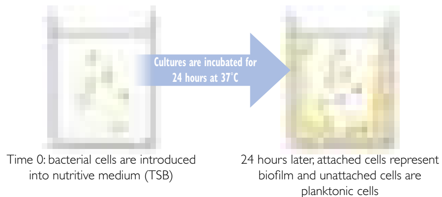
Figure 1. Biofilm formation.
