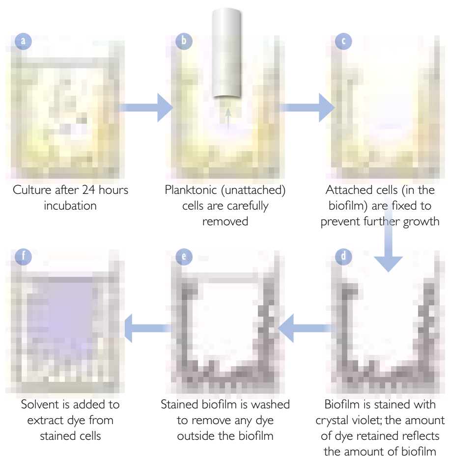
Figure 2. Biofilm evaluation.
